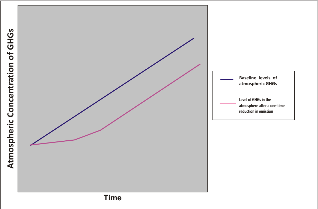
Figure 17 : Impact of a one-time reduction in emissions
