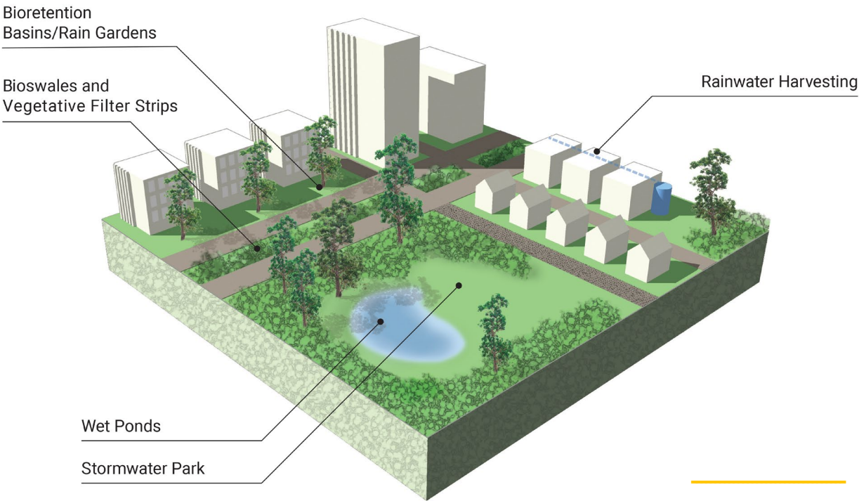
Figure 2-8. Neighborhood NBS
