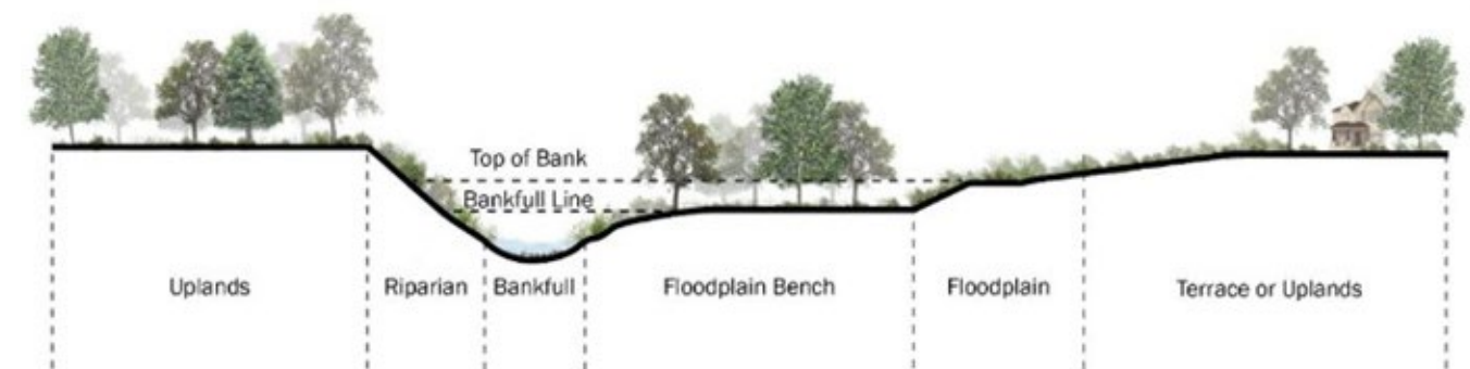
Figure 10-6. Cross section of multi-stage channel with floodplain bench 7
