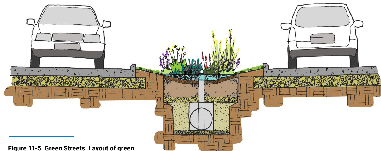
Figure 11-5. Green Streets. Layout of green streets where multiple NBS practices are combined along a roadway.
