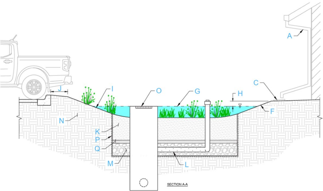
Figure 11-3. Bioretention cross section. A is drainage downspout, C is energy dissipation at flow inlet, F is vegetative groundcover, G is water surface at desired ponding depth, H is freeboard, I is side slope, J is a step out when bioretention is along the roadway, K is engineered media, L is perforated underdrain, M is drainage layer, N is embankment material, O is overflow structure, P is liner appropriate for the soil conditions, and Q is media barrier. Source: Green Infrastructure Toolkit for Texas Communities – Bioretention Design Set
