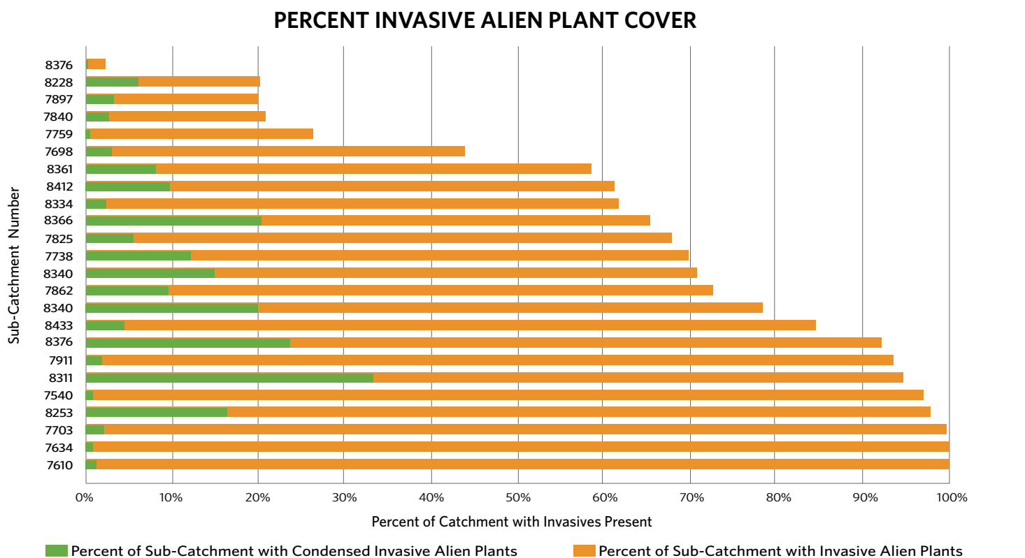
Figure 9. Invasive alien plant coverage of surface water sub-catchments, showing percentage of sub-catchment where invasive plants are present and the percentage of sub-catchment with condensed invasive plants.
