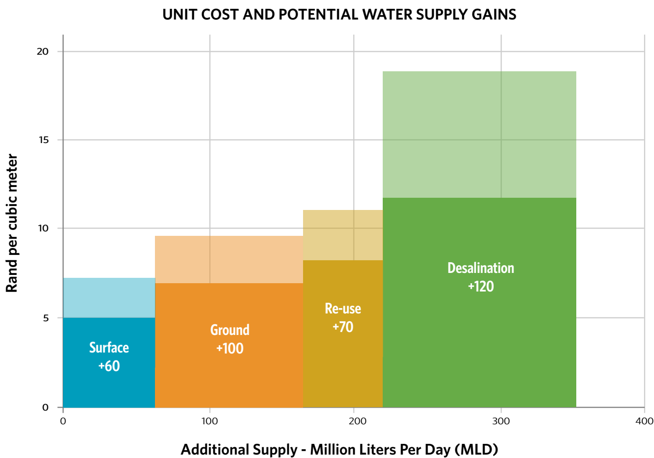
Figure 6. Unit cost comparison and estimated water yield potential of grey infrastructure solutions under consideration by the city. Significant uncertainty remains around the unit costs (shaded sections in chart). 16
