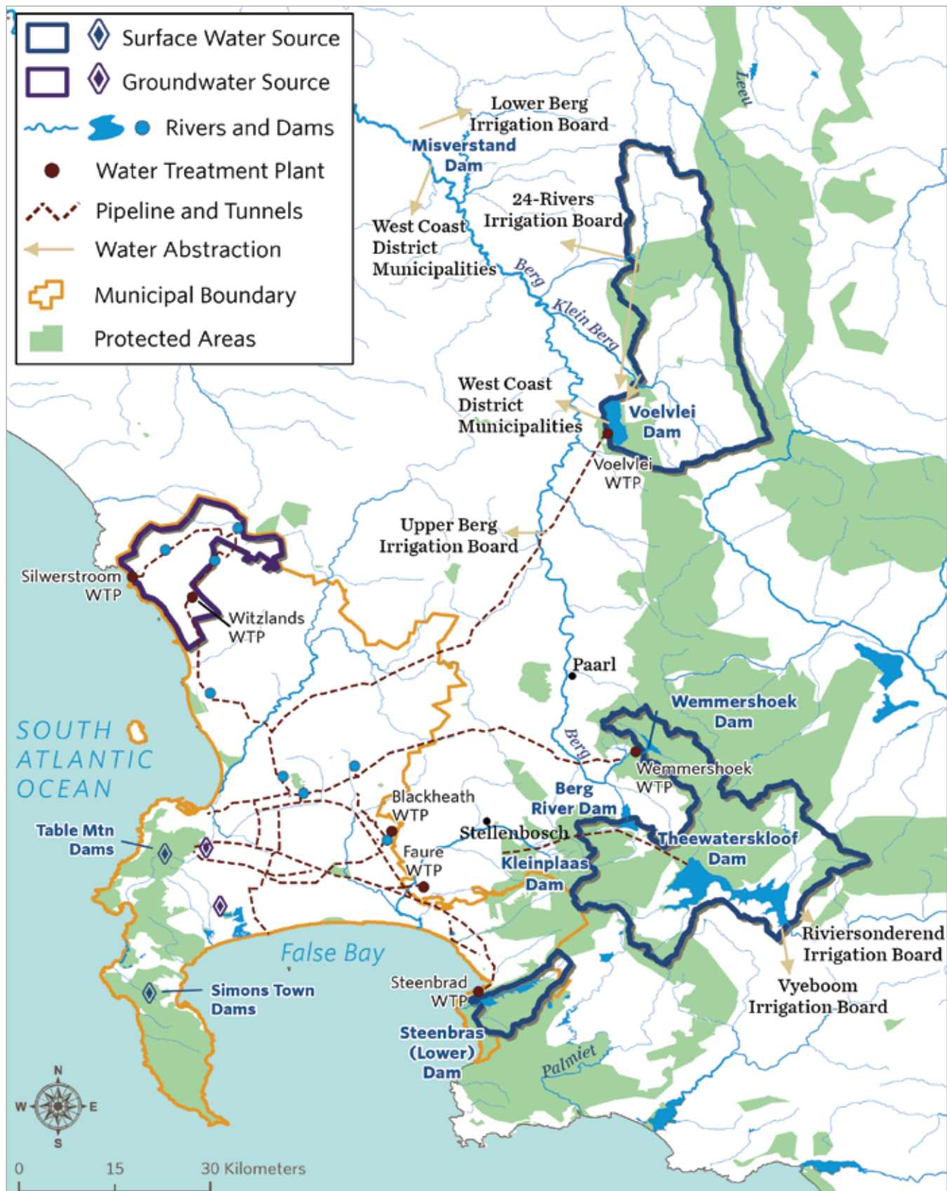
Figure 4. Western Cape Water Supply System users include the Cape Town metropolitan area, the agricultural sector, smaller municipalities, and communities. 11
