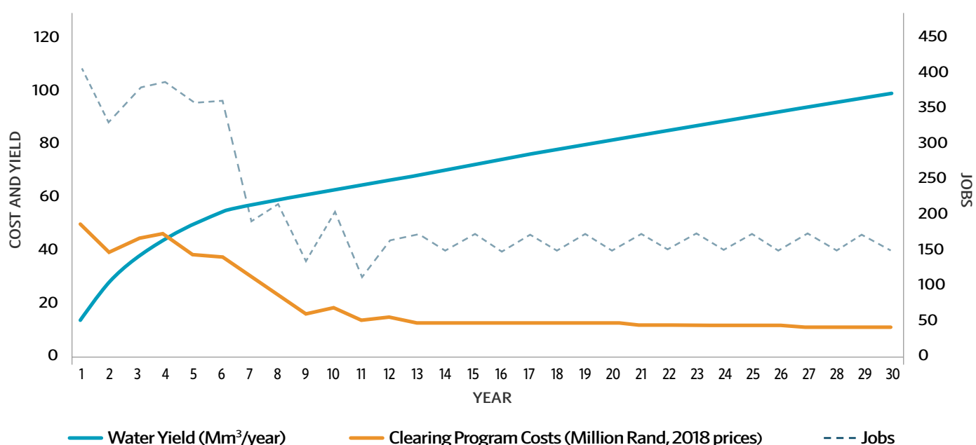
Figure 18. Discounted restoration timeline for priority sub-catchments.
