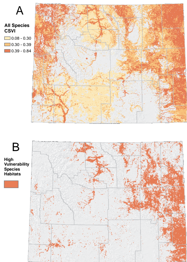
Figure 9. The cross-species vulnerability index (CSVI) was calculated across all 131 species and is displayed in three quantiles (A). High vulnerability habitats for these species were identified as those places where CSVI scores greater than 0.30 overlapped with areas of high overall landscape vulnerability (B).
