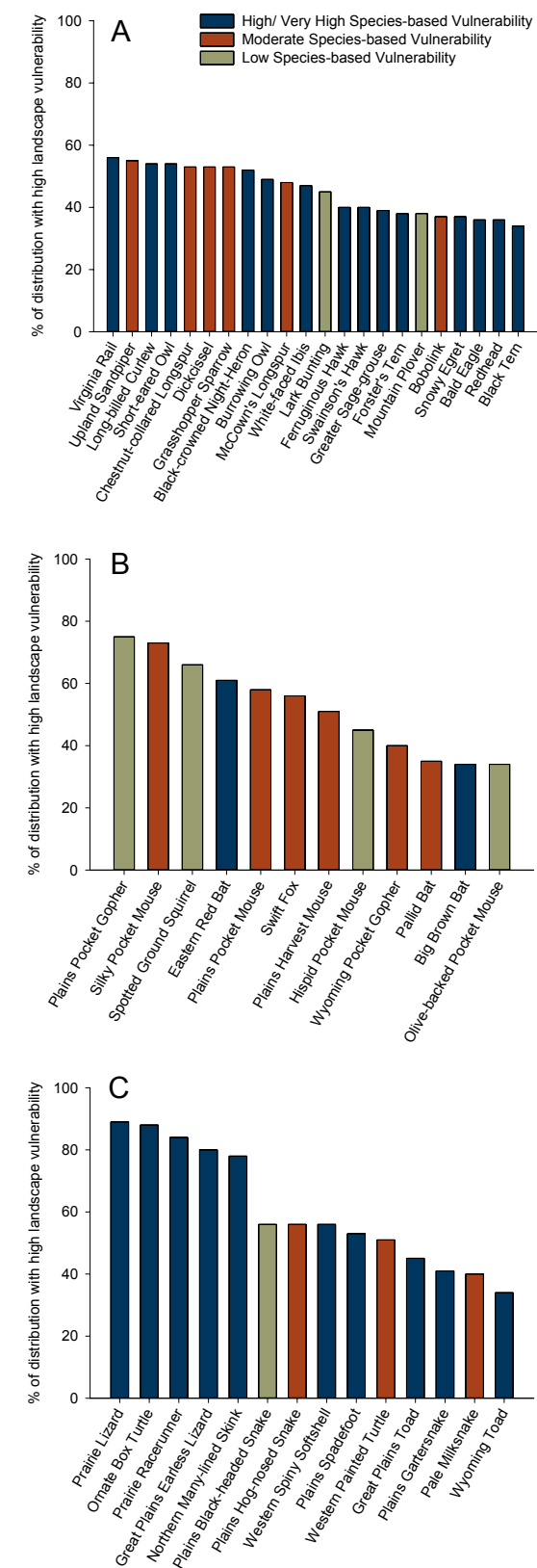
Figure 8. The 48 species ranked as highly vulnerable using the landscape-based approach, separated by birds (A), mammals (B) and amphibians and reptiles (C). The percent of each species' distribution categorized as highly vulnerable is shown on the y-axis and bar shading reflects the rank received for species-based vulnerability.
